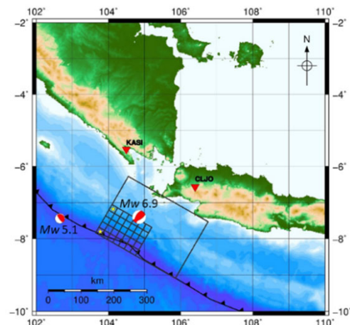
Fig. 2. Strong motion generation area estimated to simulate the M_w 8.7 hypothetical plate boundary earthquake using the M_w 5.1 plate boundary earthquake and the M_w 6.9 intraslab earthquake as the element events.
