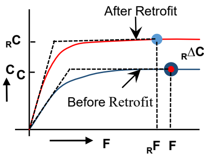
Fig. 1. The calculation procedure of required strength for retrofit. R^I_{S0} is Newly defined based on structural type after retrofit. R^{\Delta}C , new ductility index is considered which will be less than the existing F value.
